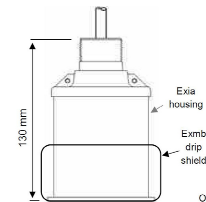
dBR Radar with submergence shield drawing
