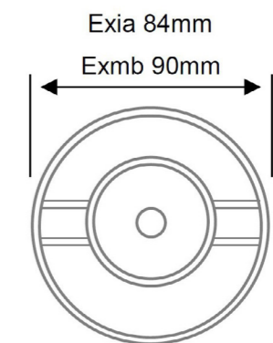
dBR Radar diameter drawing
